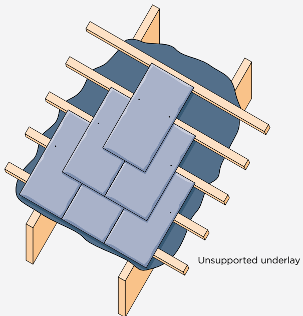
Vapour permeable underlay to BS 5534
